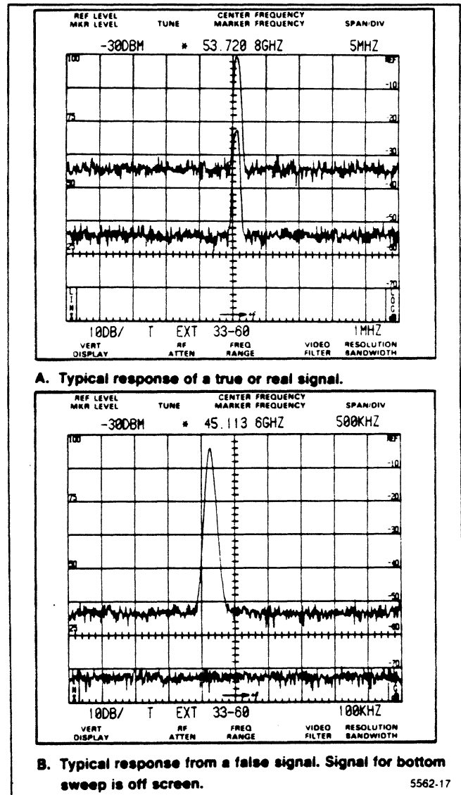
Figure 6-4. Typical example of Identifier mode displays.
